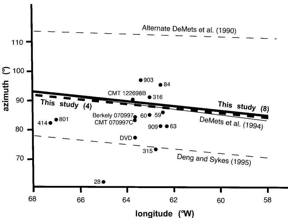
Figure 2. Predicted Caribbean–South American velocity azimuth (degrees clockwise from north) along plate boundary zone in northern South America and Trinidad at 10.5°N from this (thick lines; solid line is for eight-site Caribbean rigid-plate model; dashed line is for four-site Caribbean rigid-plate model) and previous (thin lines) studies. Four-site and eight-site Caribbean rigid-plate models both predict constant velocity magnitude of \sim 20 mm/yr across this region. Dots are slip-vector azimuths for large, upper crustal earthquakes. Numbers are event numbers in Deng and Sykes (1995) Table 1. DVD is slip vector from Doser and Van Dusen (1996) for 1929 magnitude 6.9 Cumana earthquake. Harvard CMT and Berkeley determinations for July 9, 1997, magnitude 6.8 Cariaco event and Harvard CMT determination for a December 26, 1998, event are labeled. Model labeled “Alternate DeMets et al. (1990)” omits earthquake slip vectors in Lesser Antilles. Note that Central Range fault segment of plate boundary zone in Trinidad ( \sim 61^\circ – 62^\circ W) is aseismic, whereas El Pilar fault segment in Venezuela ( \sim 62^\circ – 65^\circ W) is seismically active.
