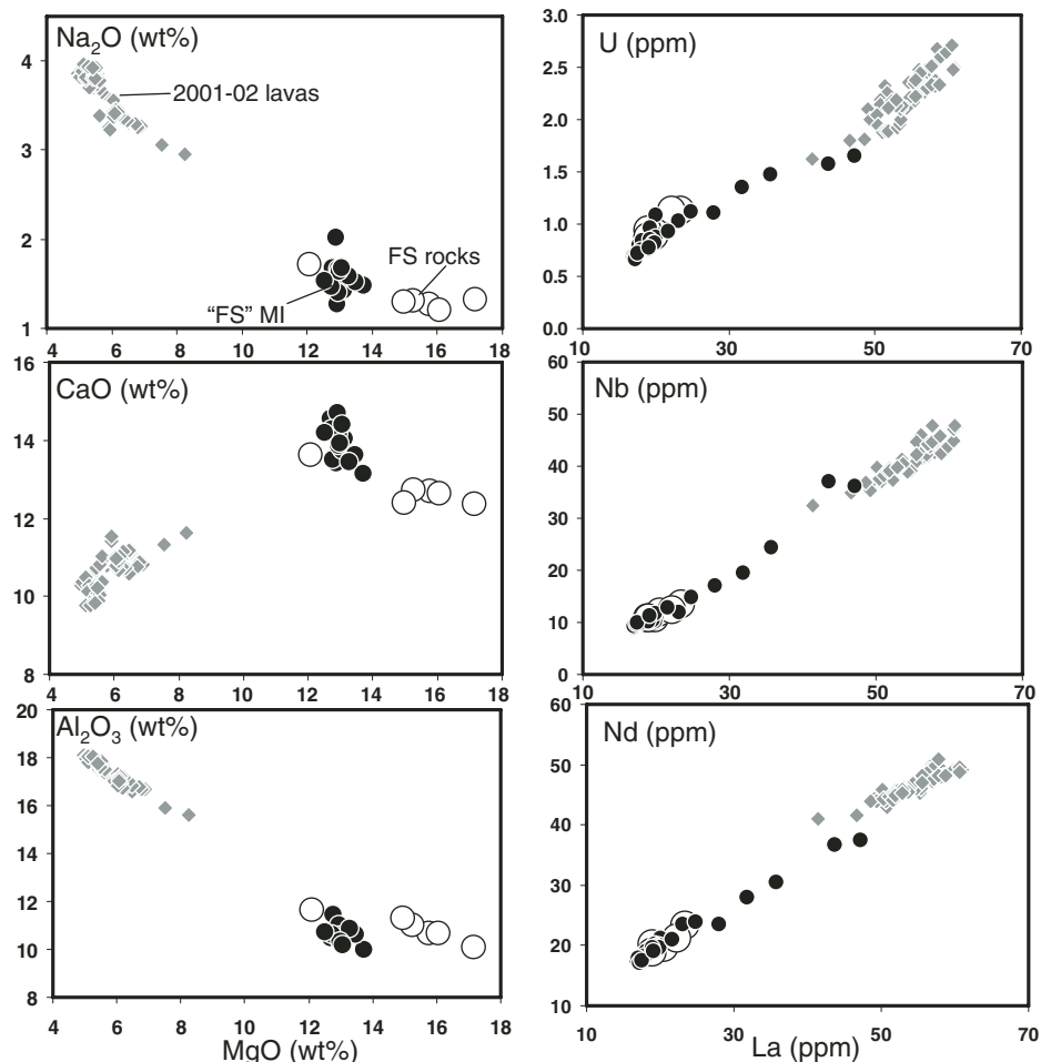
Figure 2. Comparison between compositions of fall-stratified (FS) parental magmas (exemplified by recalculated melt inclusions), FS whole rocks, and modern lavas of Mount Etna (Andronico et al., 2005; Corsaro et al., 2006). Note significant variations in trace elements among individual melt inclusions. Symbols as in Figure 1.
