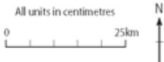
Oct 14, 1974 Tephra Deposit
