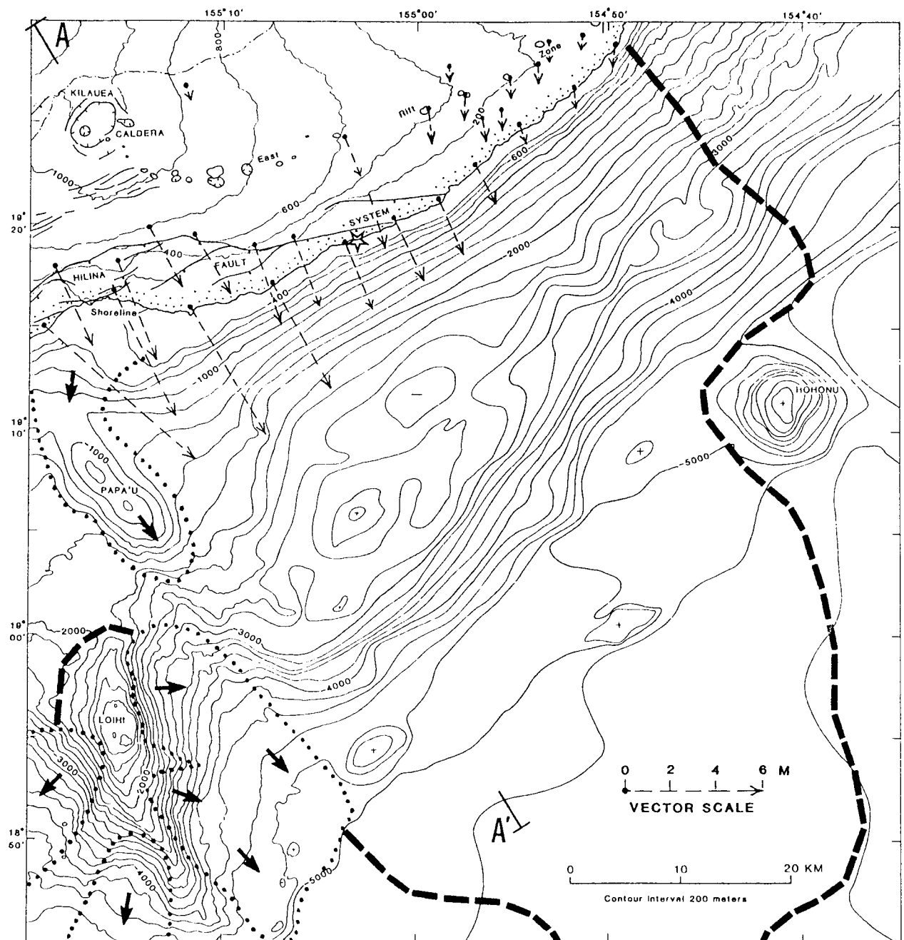
Fig. 10. Bathymetric-topographic map of the Hilina slump area. Bathymetry from National Ocean Survey [1981, 1982] and land contours from USGS 1:100,000 topographic map. Contour interval is 200 m. Heavy dashed line is margin of Hilina slump, and dotted lines bound smaller overriding Papa'u and Loihi landslides with movement direction shown by short arrows. Dash-dotted line is boundary between Kilauea volcano and Mauna Loa volcano to north. The epicenter of the magnitude 7.2 (1975) earthquake is shown by star, and dashed arrows are geodetically measured vectors showing horizontal movement associated with the earthquake [after Lipman et al. , 1985]. A-A' indicates location of section of Figure 11.
