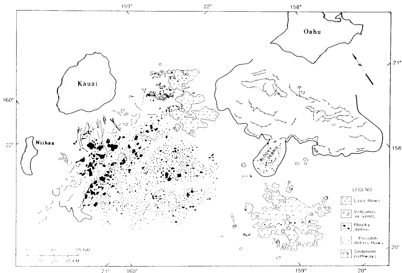
Fig. 5. Tracing from GLORIA image showing contrasting features of the South Kauai debris avalanche and the Waianae slump.
