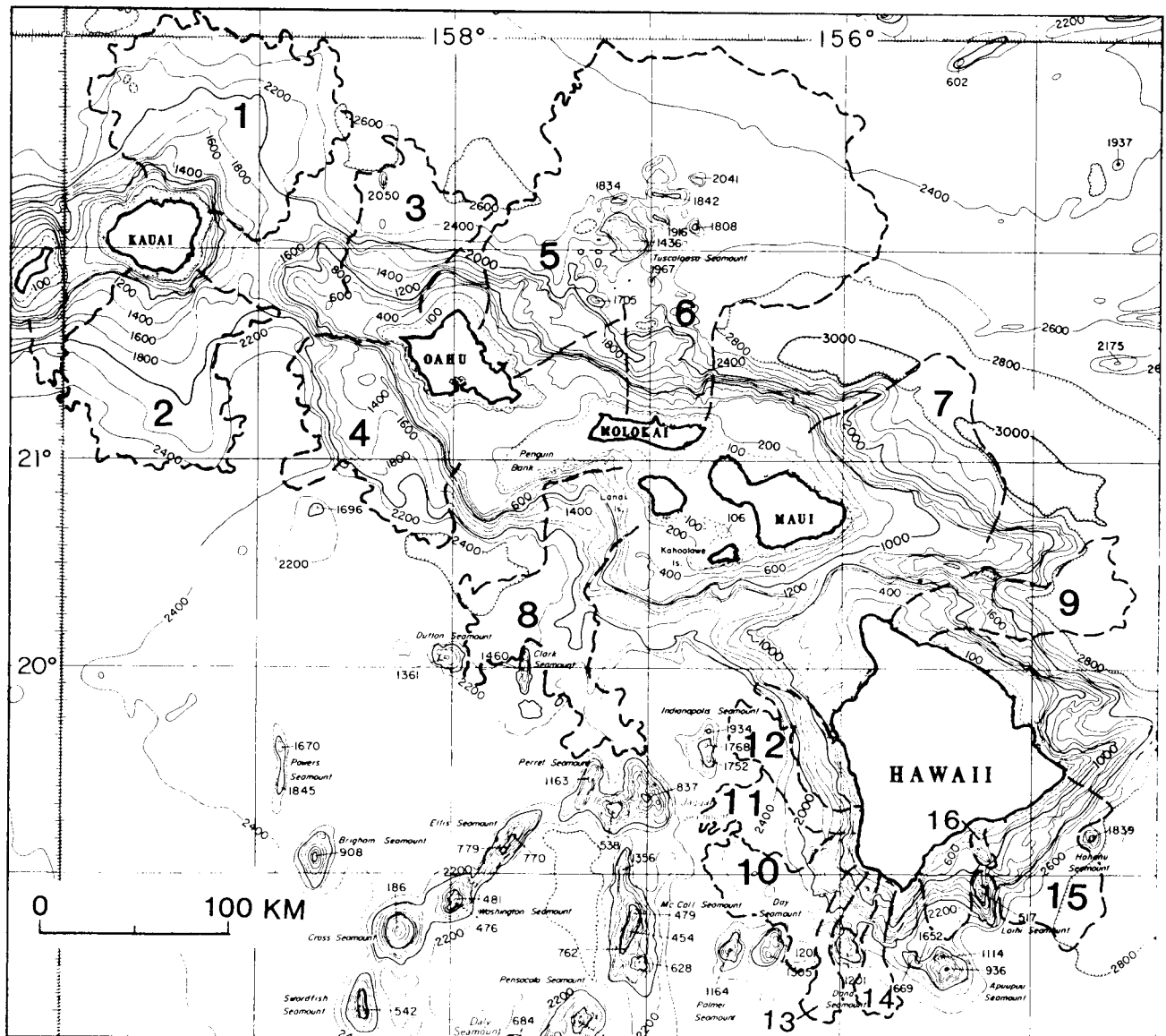
Fig. 1. Bathymetric map of the southeastern Hawaiian Ridge showing major mass wasting features (heavy dashed lines) identified by number in text and Table 1. Contour interval 200 fathoms (366 m). Base from U.S. Naval Oceanographic Office [1973].
