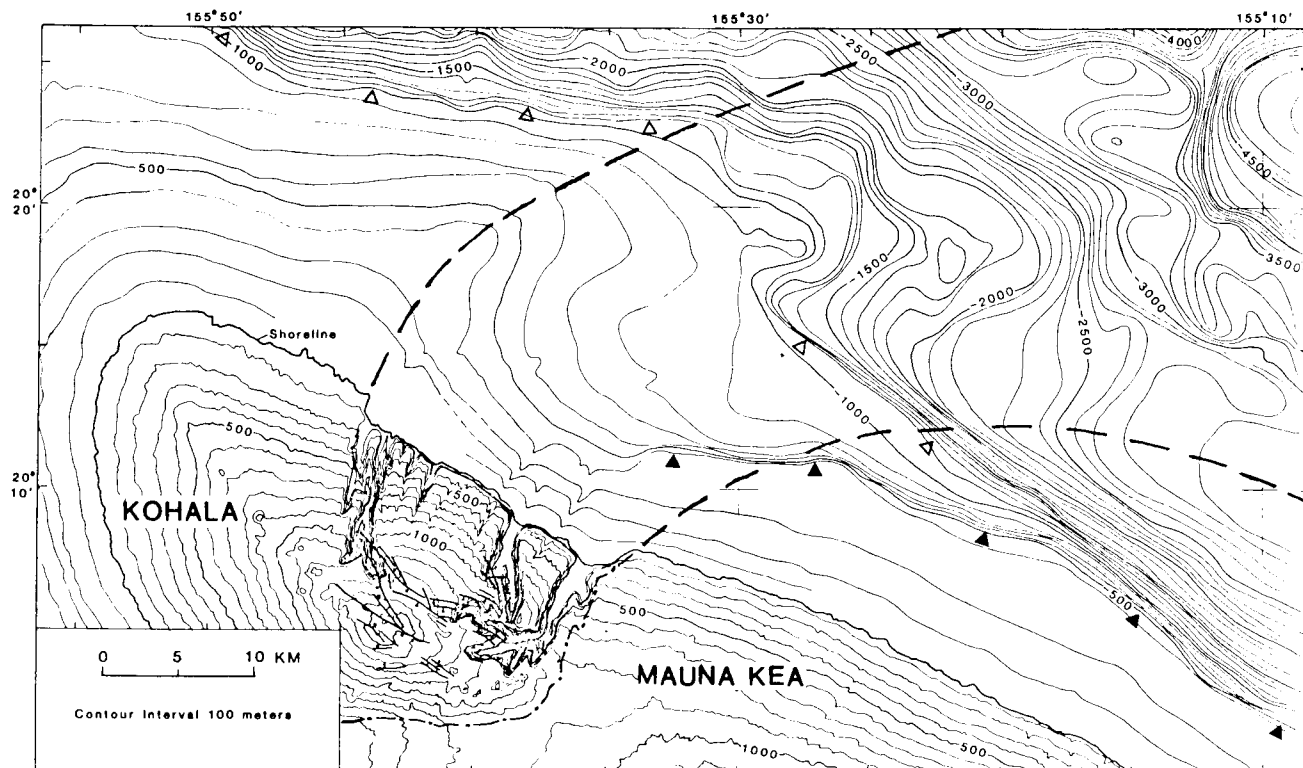
Fig. 9. Bathymetric-topographic map of the upper part of the Pololu debris avalanche (margins shown by dashed line). Also shown are the edge of Mauna Kea lava flows lapping onto Kohala volcano (dash-dotted line), the Kohala shelf break (open triangles), and the Mauna Kea shelf break (solid triangles). Bathymetry south of 20°22' contoured from National Ocean Survey [1981] and north of 20°22' from Campbell [1987], and land contours from USGS 1:100,000 1980 topographic map. Contour interval above and below sea level is 100 m.
