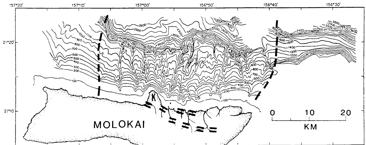
Fig. 8. Bathymetry north of Molokai from A. Malahoff and C. D. Hollister (written communication, 1987); contour interval 100 m. Margins of the Wailau debris avalanche shown by heavy dashed lines and trend of dike swarms is shown by double dashed lines [from Stearns and Macdonald , 1947]. Note that major canyons above sea level (shown by curved lines) are commonly aligned with submarine canyons. The postslide Kalaupapa volcano (K) grew in the slide amphitheater after subsidence was complete and partly filled the upper part of adjacent, submerged canyons.
