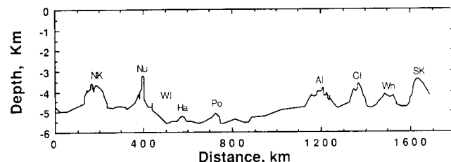
Fig. 12. Bathymetric profile along axis of Hawaiian Deep proceeding clockwise from the north side of Kauai, around the island of Hawaii, and northwest to the south side of Kauai (see Figure 2 for location). Humps produced by distal parts of landslides are North Kauai (NK), Nuananu (Nu), Wailau (WI), Hana (Ha), Pololu (Po), Alikai (Al), Clark (Cl), Waianae (Wn), and South Kauai (SK).
