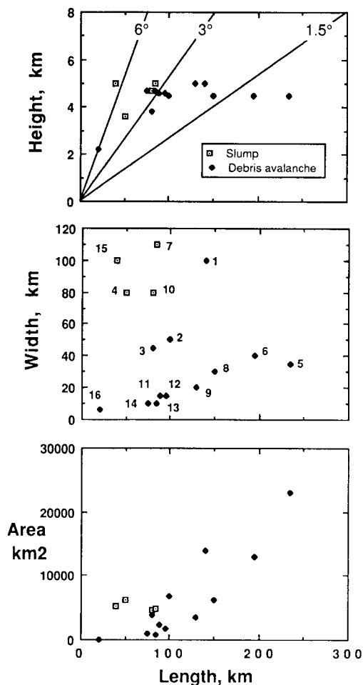
Fig. 4. Length versus height, width, and area for large Hawaiian slumps and debris avalanches identified by number in text and Table 1. Height is measured from toe to sea level; lines show overall gradient in degrees. Width of the head of the landslide and area are measured below sea level.
