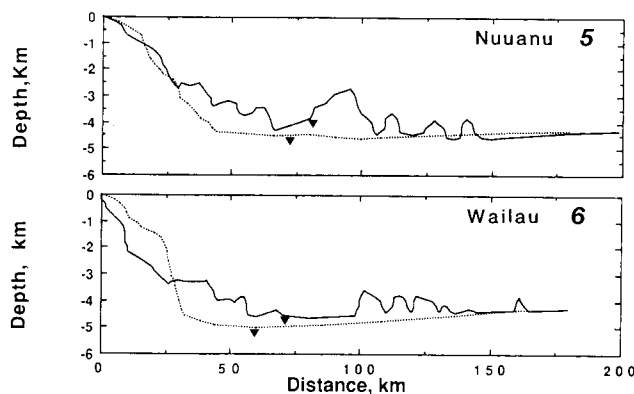
Fig. 6. Longitudinal profiles from Nuuanu and Wailau debris avalanches. Dotted profiles are on northwest margin of Nuuanu and east margin of Wailau landslides. Projected trace of Hawaiian Deep axis shown by triangles. See Figure 2 for location. Vertical exaggeration is 10.
