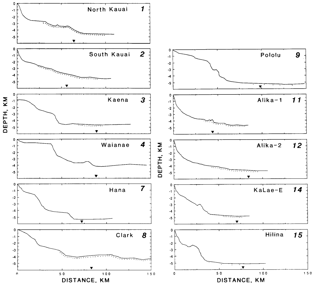
Fig. 3. Longitudinal profiles of landslides as numbered in Table 1 and shown in Figures 1 and 2. Hummocky terrain is indicated by dots (widely spaced where faintly visible), and lower end of dots is known lower limit of debris avalanche. Projected trace of Hawaiian Deep axis shown by triangle. Vertical exaggeration is 7.5.
