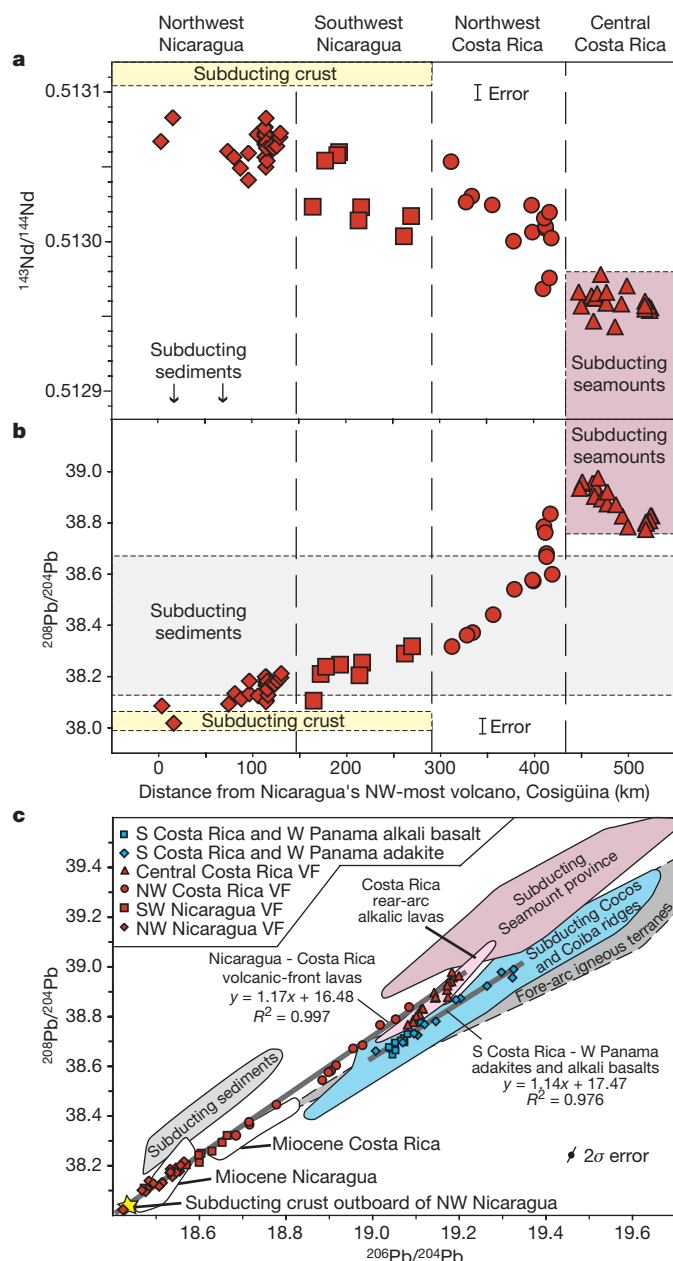
Figure 2 | Systematic variation in lead and neodymium isotopic composition along the volcanic front from Costa Rica to northwest Nicaragua indicates northwestward flow of mantle wedge material.
