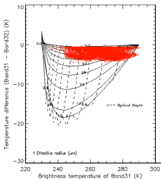
Figure 3. The temperature difference and brightness temperatures at 11.03 μm for individual pixel values (red dots) in MODIS data indicating a large proportion of pixels with negative BTM values.
