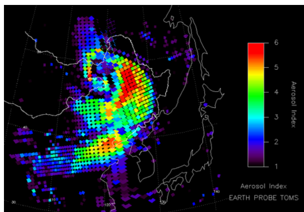
Figure 2b. TOMS ultraviolet aerosol index image on April 07, 2001. The Chinese dust cloud is observed in two orbits at 01:45 UTC and 03:23 UTC respectively. High AI values, which represent larger amount of silicate aerosol in the cloud, show a similar pattern to the infrared image in Figure 2a.
